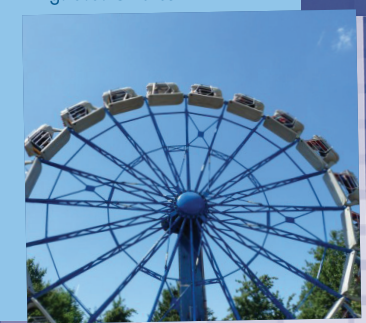
Fig. 3.8: G-Force
